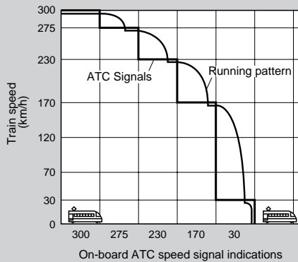
Figure 5 ATC Train Running Pattern
