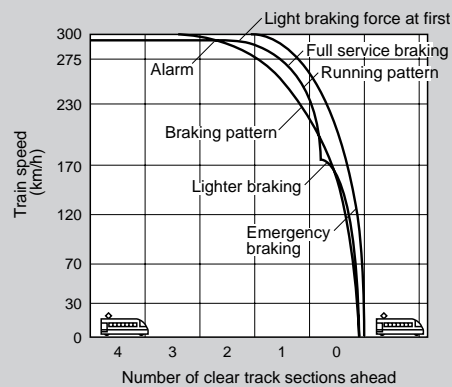
Figure 6 Digital ATC Train Running Pattern
