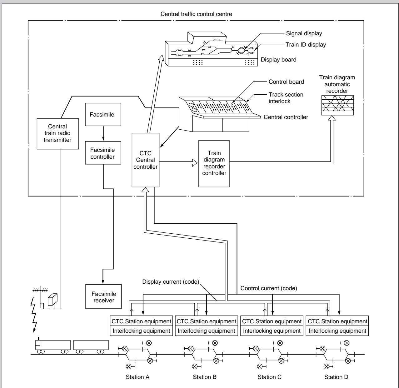
Figure 8 CTC System
