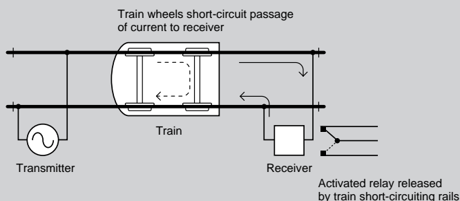
Figure 1 General Principles of Track Circuit
