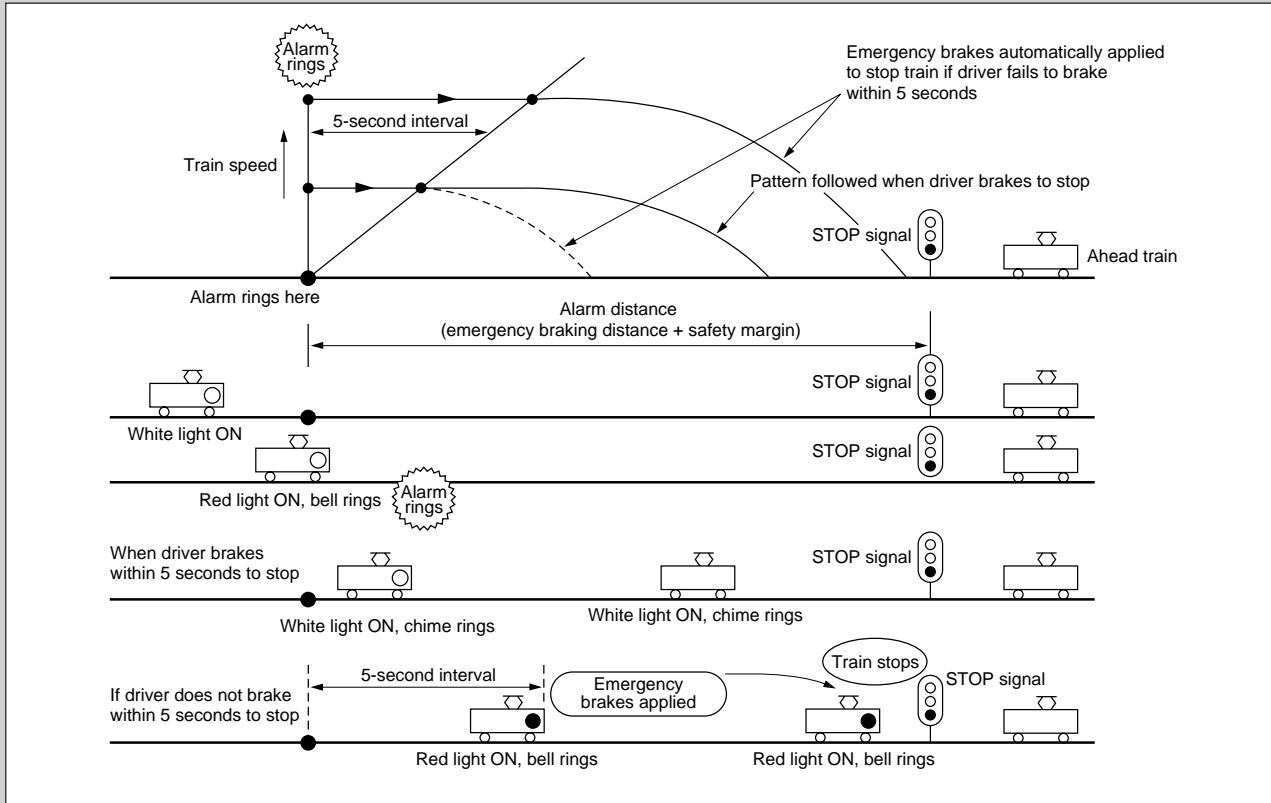
Figure 3 Operation of ATS-S System
