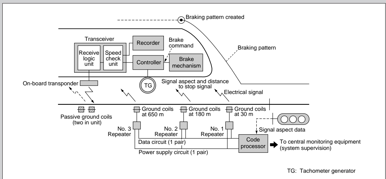
Figure 4 Operation of ATS-P System
