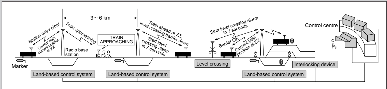
Figure 7 CARAT System
