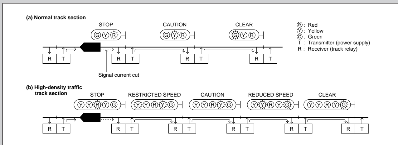
Figure 2 Automatic Block Signalling System
